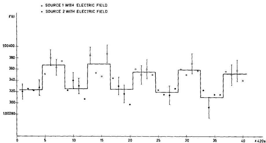
Fig. 3. The step method : The value for 2 \Delta\lambda/\lambda is (40 \pm 4) \times 10^{-5} at an external electric field strength of 1.2 \times 10^4 V/cm. The \text{NaTcO}_4 source was prepared by method I.
