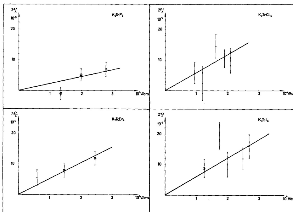
Fig. 5. Results of 2 \Delta\lambda/\lambda at different external electric field strengths for the Tc-halogen complexes. The results marked \odot are averages of two measurements.
