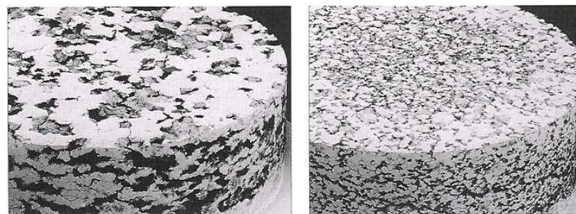
Fig. 8. Matrix-controlled release system [16] after erosion of 60% (w/w) of well soluble caffeine from an ethylcellulose matrix
