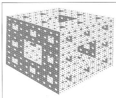
Fig. 7. Menger sponge with a fractal dimension of 2.63 [15]
